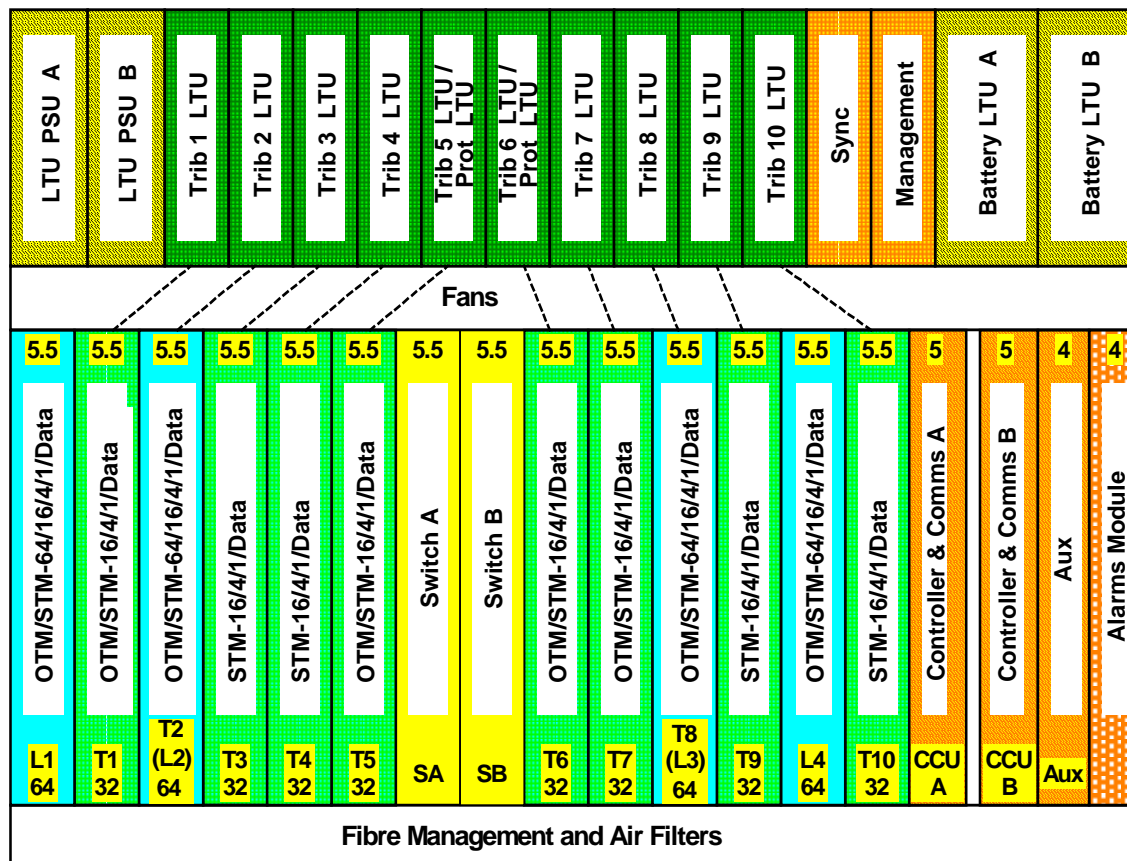
Figure 4: OMS3240 Subrack layout
