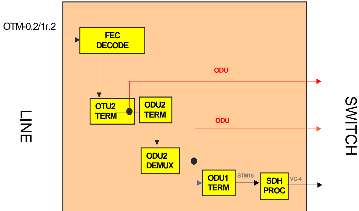
Figure 7: features provided by the OTM-0.2/1r.2 card
