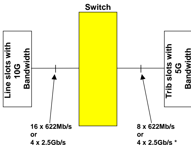
Figure 8: OMS3240 Transmission of payload to switch via backplane
