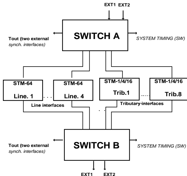
Figure 17: OMS3240 Distribution of Timing Signals
