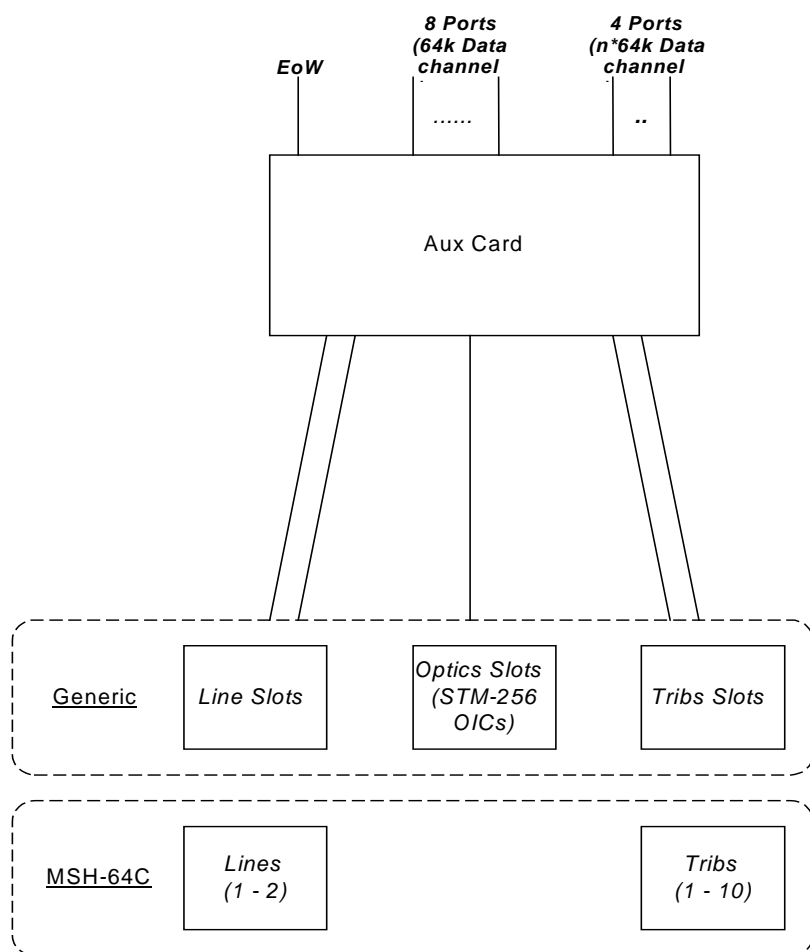
Figure 19: Distribution of OH Bytes
