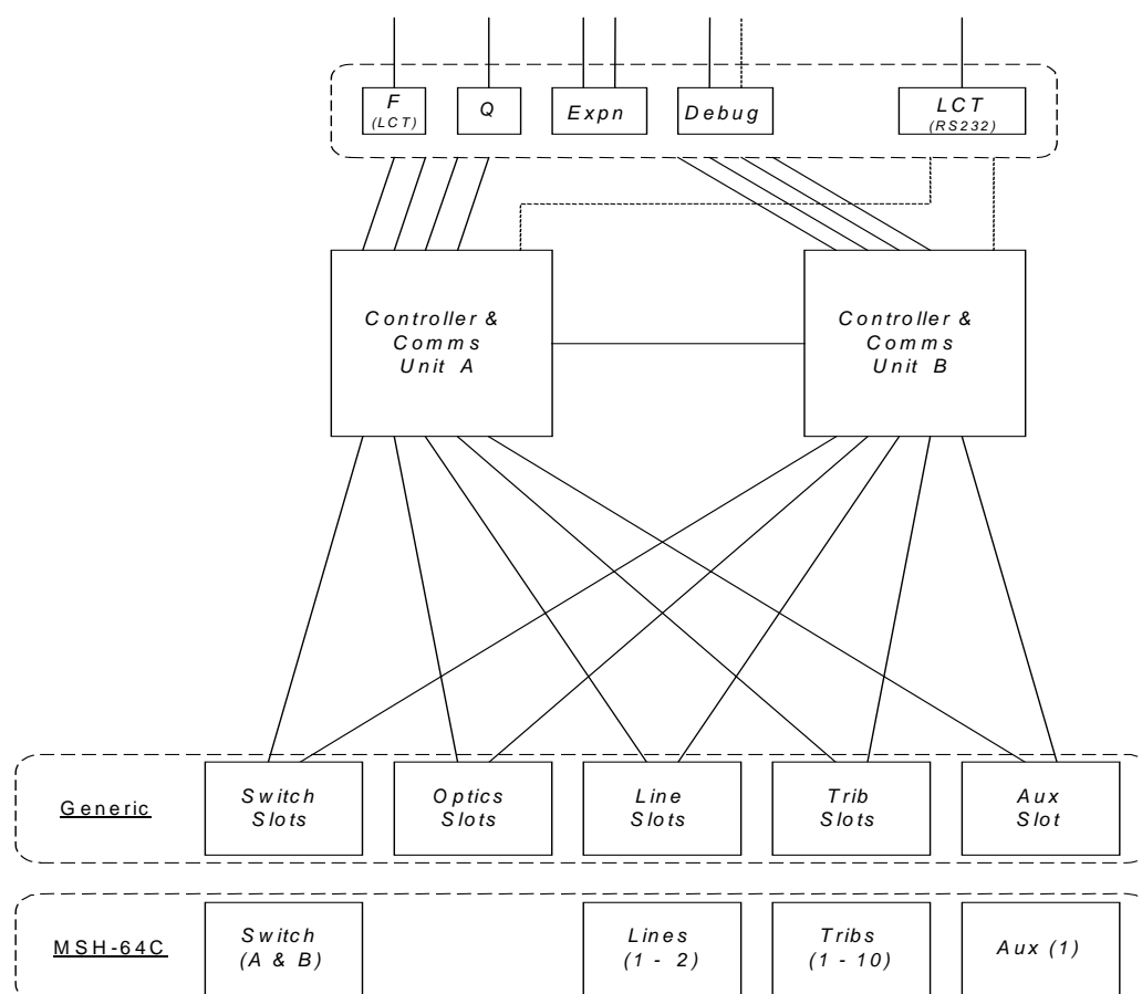
Figure 18: Distribution of Control Signals
