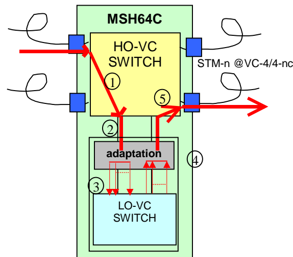
Figure 11: Processing inside the LO Stitching matrix
