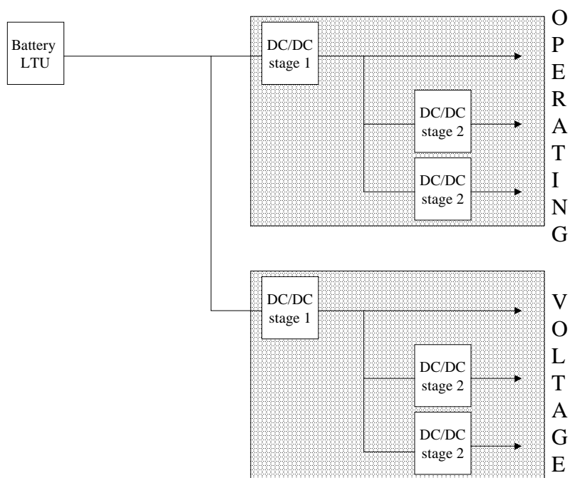
Figure 20: Power Supply Distribution
