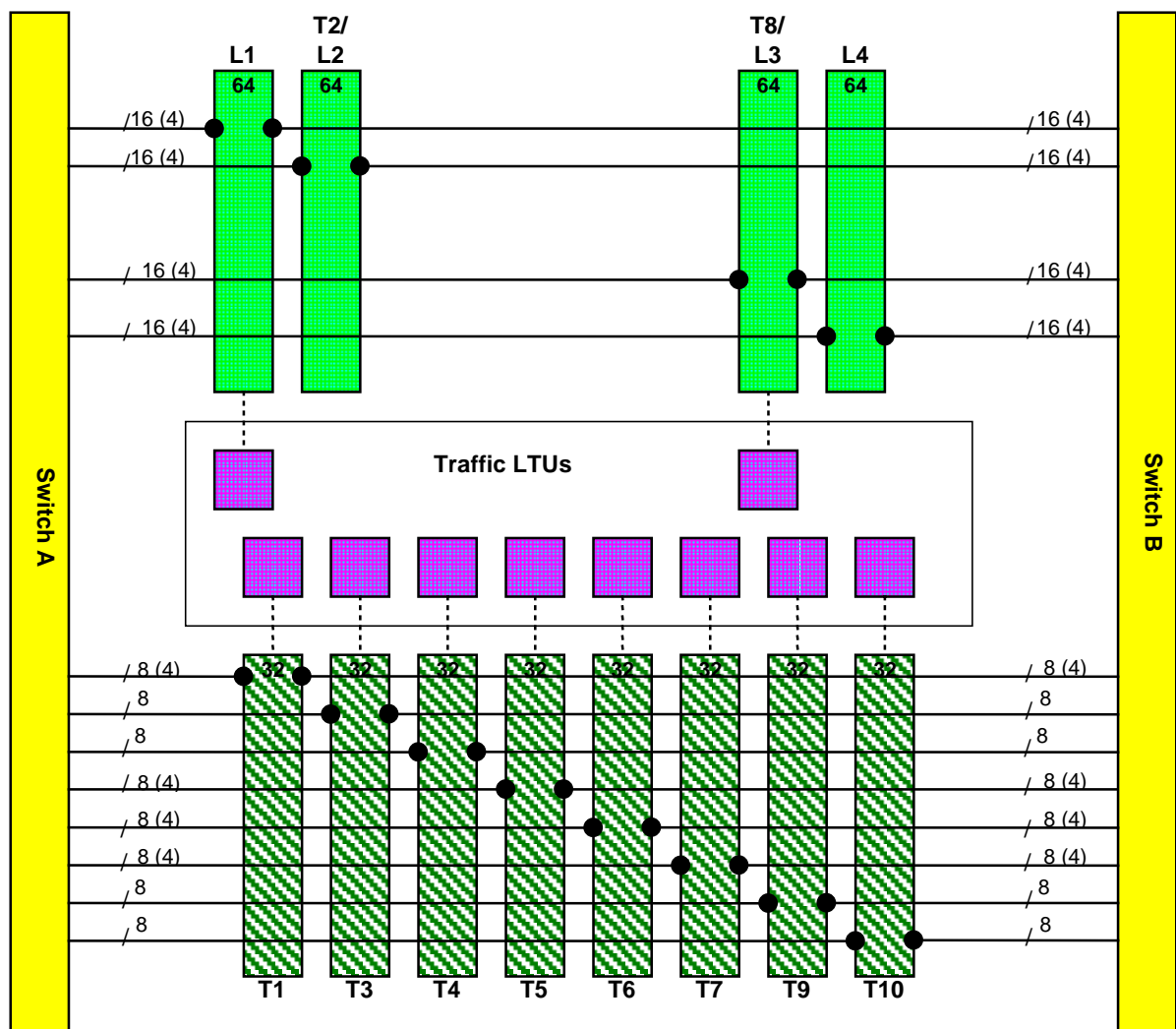
Figure 16: Distribution of Traffic Signals using 622Mb/s (or 2.5Gb/s) LVDS links
