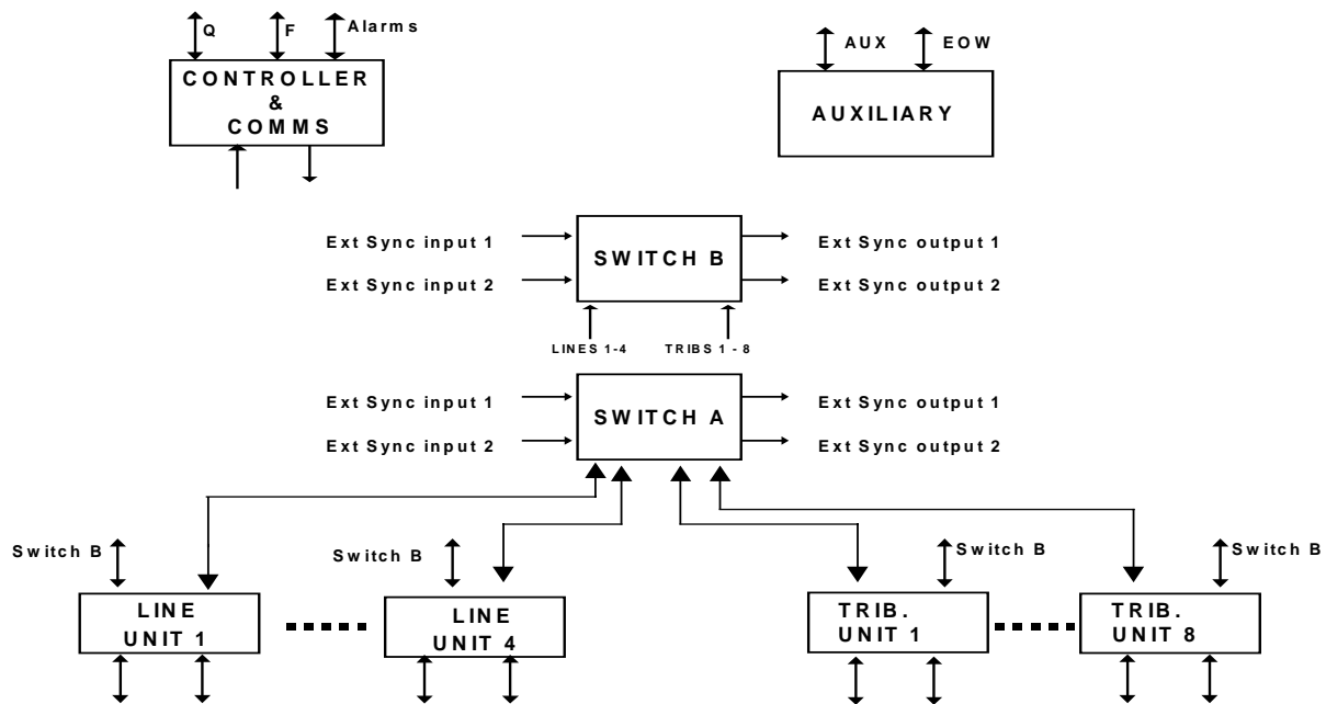
Figure 15: OMS3240 General Block Diagram
