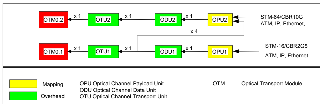
Figure 3: OTN (Optical Transport Network) structure according to ITU-T G.709
